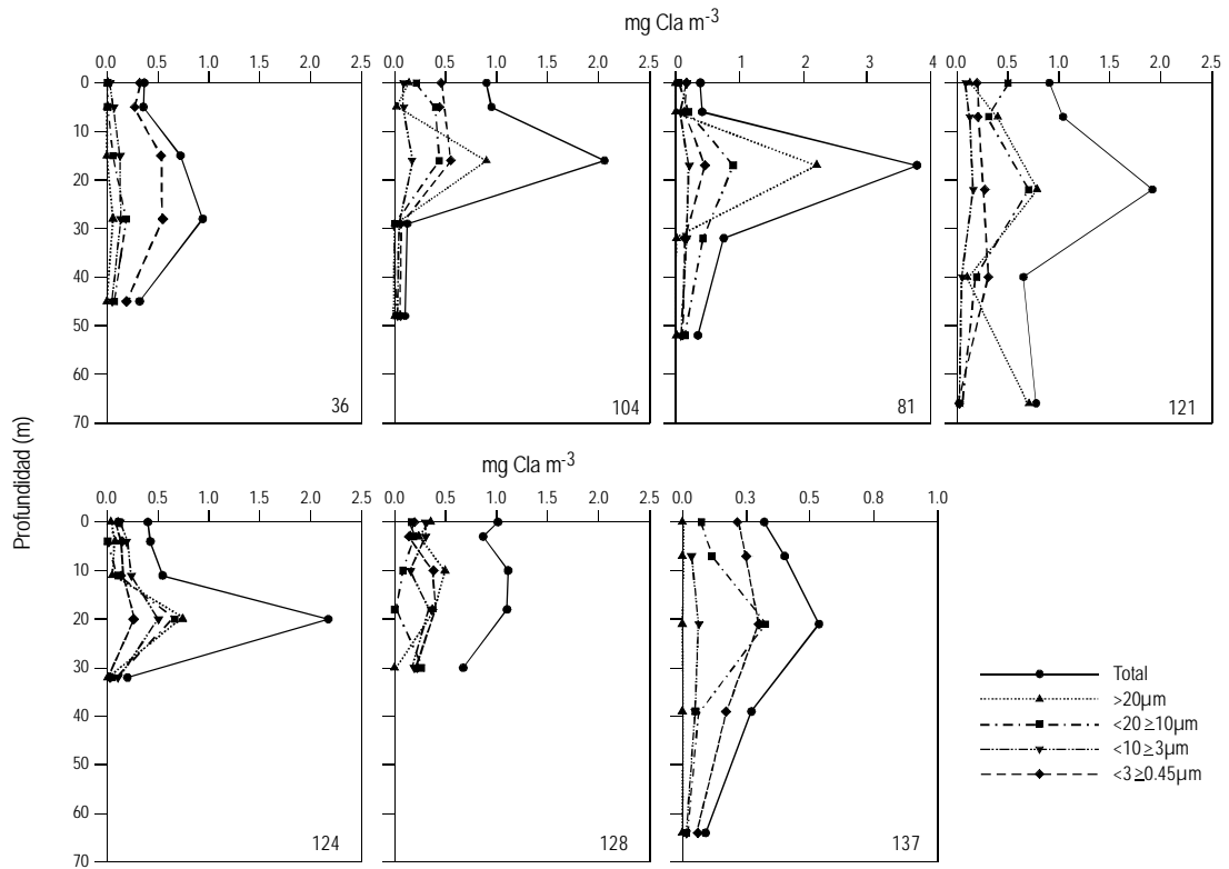
Figura 4. Distribuciones verticales de clorofila \alpha . Figure 4. Vertical distribution of chlorophyll \alpha .
