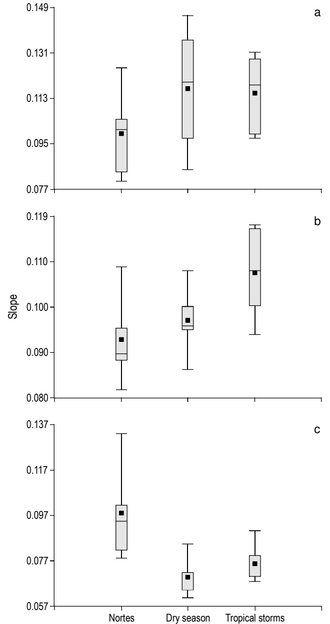
Figure 4. Swash zone slope at each of the study sites (A, B, C) and per season. The Nortes season lasts from October to February, the dry season from March to May, and the tropical storm season from June to November.
