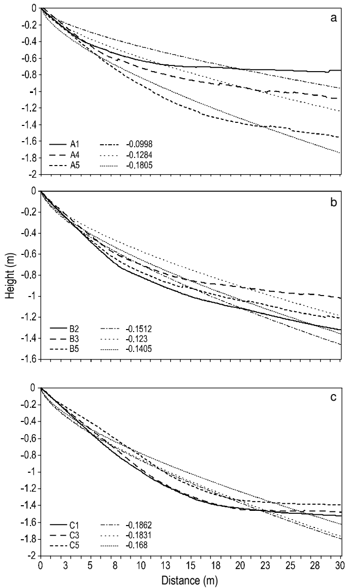
Figure 3. Mean profile of the swash and surf zones of the three zones surveyed (A, B, and C) using the equilibrium profile equation: h = Ax^{2/3} . The value of parameter A is shown for the profiles plotted.
