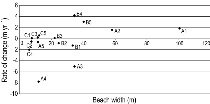
Figure 6. Beach width on the last date recorded (July 2006) and rate of change in shoreline position.
