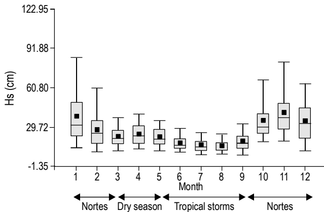
Figure 8. Monthly mean significant wave heights.
