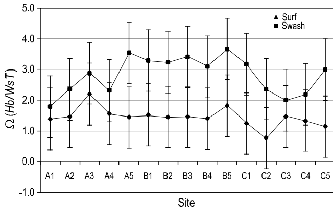
Figure 9. Spatial variability of the \Omega parameter along the coast for the swash and surf zones. Mean values and standard errors are shown.
