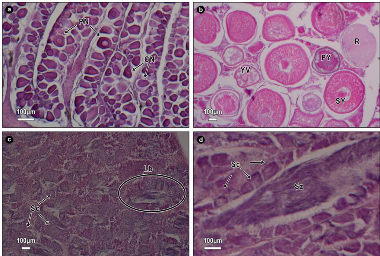
Figure 3. Transverse section of the ovary (a, b) and testis (c, d) of Scomberomorus sierra . (a) Immature ovary with oocytes in previtellogenesis (40×) and (b) ripe ovary showing oocytes in several stages of development: chromatin-nucleolus (CN), perinucleolus (PN), yolk vesicle (YV), primary yolk (PY), secondary yolk (SY), and ripe (R) (10×). (c) Immature testis: spermatocysts (Sc) and lobules with poor development (Lb) (10×). (d) Ripe testis: spermatocysts (Sc) around lobule and lobular lumen filled with spermatozoa (Sz) (40×).
