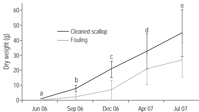
Figure 3. Variation of fouling and cleaned scallop dry weight between June 2006 and July 2007 in the Nodipecten nodosus culture at Canto Grande, Santa Catarina, Brazil (different letters indicate significant difference between sampling periods).
