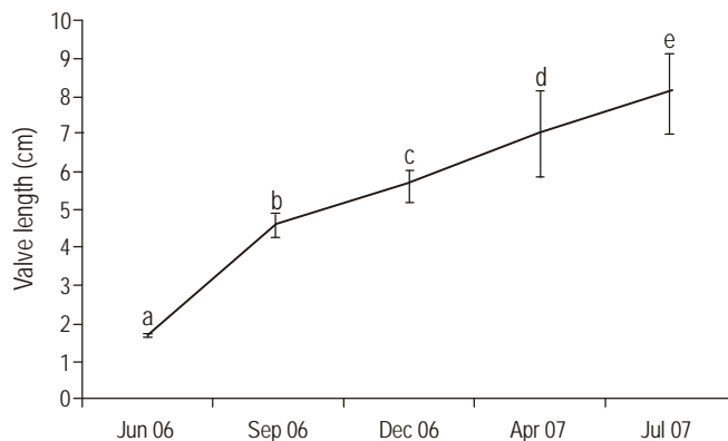
Figure 4. Scallop growth in shell length from June 2006 to July 2007 in the Nodipecten nodosus culture at Canto Grande Beach, Santa Catarina, Brazil (different letters indicate significant difference between sampling periods).
